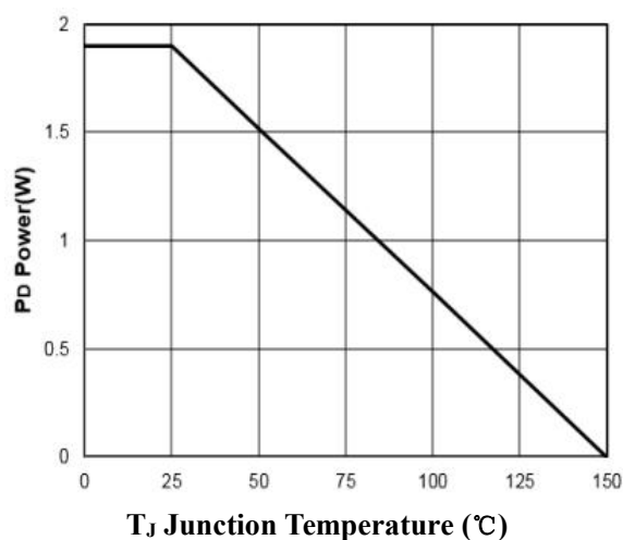
Figure 8: Power Dissipation
